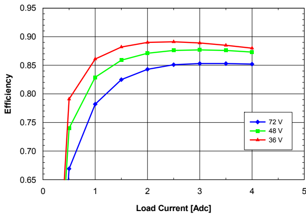
Fig. 12V.5: Efficiency vs. load current and input voltage for SQ48T/S04120 converter mounted vertically with air flowing from pin 3 to pin 1 at a rate of 300 LFM (1.5 m/s) and T_a = 25\text{ }^{\circ}\text{C} .
