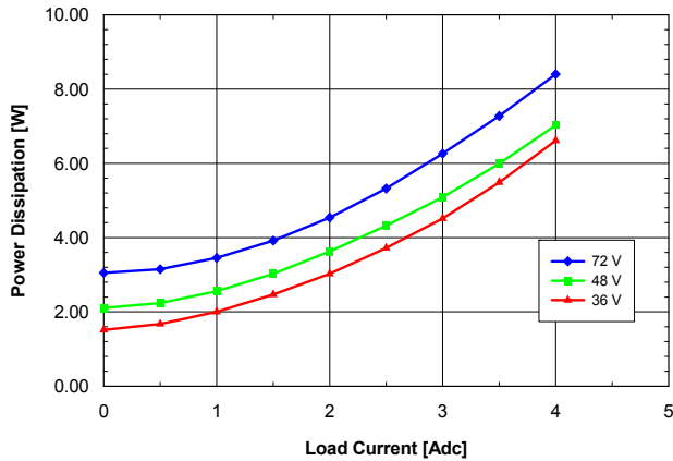
Fig. 12V.7: Power dissipation vs. load current and input voltage for SQ48T/S04120 converter mounted vertically with air flowing from pin 3 to pin 1 at a rate of 300 LFM (1.5 m/s) and T_a = 25\text{ }^\circ\text{C} .
