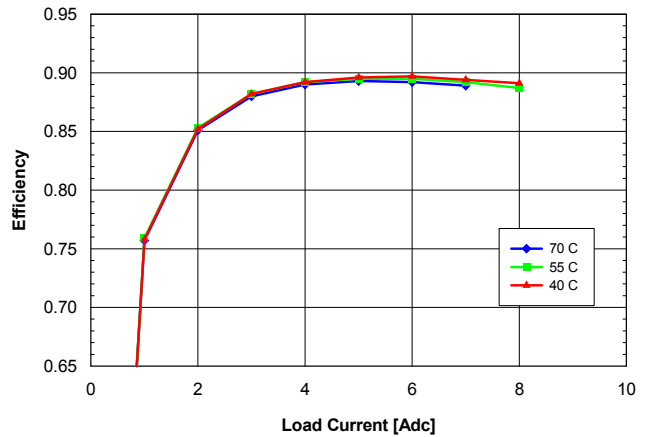
Fig. 6.0V.6: Efficiency vs. load current and ambient temperature for SQ48T/S08060 converter mounted vertically with V_{in} = 48\text{ V} and air flowing from pin 3 to pin 1 at a rate of 200 LFM (1.0 m/s).
