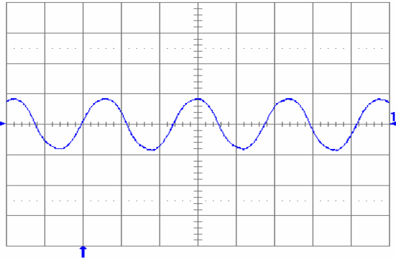
Fig. 12V.13: Output voltage ripple (50 mV/div.) at full rated load current into a resistive load with C_o = 10 \mu F tantalum + 1 \mu F ceramic and V_{in} = 48 V. Time scale: 1 \mu s/div.
