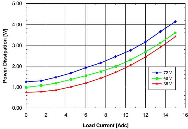
Fig. 1.0V.7: Power dissipation vs. load current and input voltage for SQ48T/S15010 converter mounted vertically with air flowing from pin 3 to pin 1 at a rate of 300 LFM (1.5 m/s) and T_a = 25\text{ }^\circ\text{C} .
