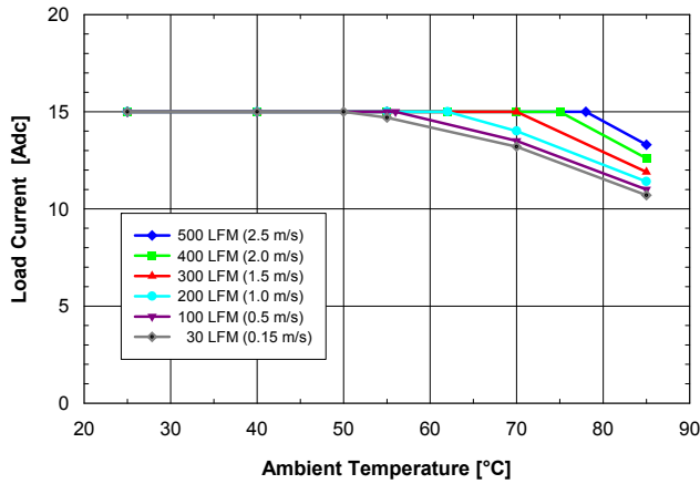
Fig. 3.3V.3: Available load current vs. ambient air temperature and airflow rates for SQ48S15033 converter mounted vertically with V_{in} = 48\text{ V} , air flowing from pin 3 to pin 1, and maximum FET temperature \leq 120\text{ }^\circ\text{C} .
