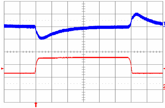
Fig. 5.0V.11: Output voltage response to load current step-change (2.5 A – 5 A – 2.5 A) at V_{in} = 48 V. Top trace: output voltage (200 mV/div.). Bottom trace: load current (2 A/div.). Current slew rate: 0.1 A/ \mu s. C_o = 1 \mu F ceramic. Time scale: 0.2 ms/div.
