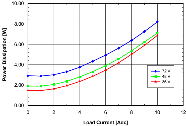
Fig. 5.0V.7: Power dissipation vs. load current and input voltage for SQ48T/S10050 converter mounted vertically with air flowing from pin 3 to pin 1 at a rate of 300 LFM (1.5 m/s) and T_a = 25\text{ }^\circ\text{C} .
