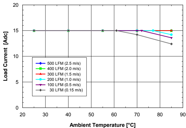
Fig. 1.8V.2: Available load current vs. ambient air temperature and airflow rates for SQ48T15018 converter with D height pins mounted horizontally with V_{in} = 48\text{ V} , air flowing from pin 3 to pin 1, and maximum FET temperature \leq 120\text{ }^\circ\text{C} .
