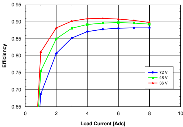
Fig. 6.0V.5: Efficiency vs. load current and input voltage for SQ48T/S08060 converter mounted vertically with air flowing from pin 3 to pin 1 at a rate of 300 LFM (1.5 m/s) and T_a = 25\text{ }^{\circ}\text{C} .
