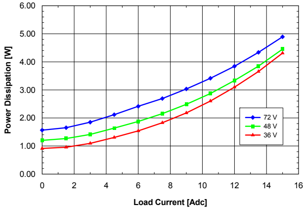
Fig. 1.8V.7: Power dissipation vs. load current and input voltage for SQ48T/S15018 converter mounted vertically with air flowing from pin 3 to pin 1 at a rate of 300 LFM (1.5 m/s) and T_a = 25\text{ }^\circ\text{C} .
