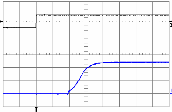
Fig. 12V.9: Turn-on transient at full rated load current (resistive) with no output capacitor at V_{in} = 48\text{ V} , triggered via ON/OFF pin. Top trace: ON/OFF signal (5 V/div.). Bottom trace: output voltage (5 V/div.). Time scale: 1 ms/div.
