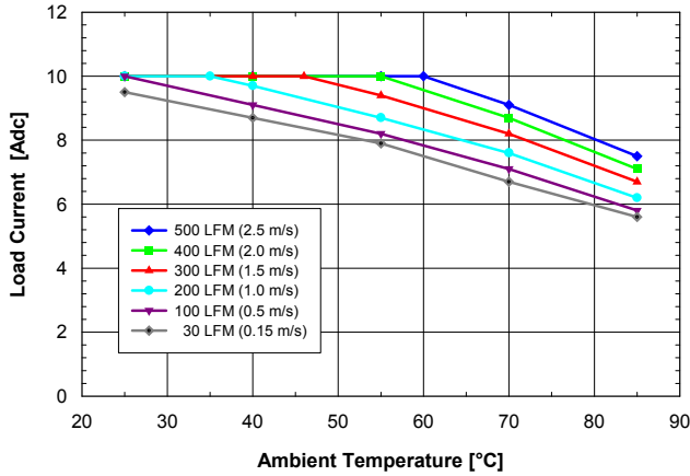
Fig. 5.0V.3: Available load current vs. ambient air temperature and airflow rates for SQ48S10050 converter mounted vertically with V_{in} = 48\text{ V} , air flowing from pin 3 to pin 1, and maximum FET temperature \leq 120\text{ }^{\circ}\text{C} .
