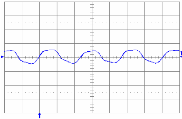
Fig. 6.0V.13: Output voltage ripple (50 mV/div.) at full rated load current into a resistive load with C_o = 10 \mu F tantalum + 1 \mu F ceramic and V_{in} = 48 V. Time scale: 1 \mu s/div.
