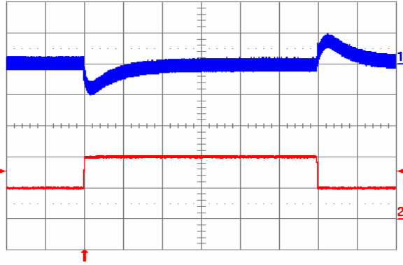
Fig. 12V.11: Output voltage response to load current step-change (1 A – 2 A – 1 A) at V_{in} = 48 V. Top trace: output voltage (200 mV/div.). Bottom trace: load current (1 A/div.). Current slew rate: 0.1 A/ \mu s. C_o = 1 \mu F ceramic. Time scale: 0.5 ms/div.
