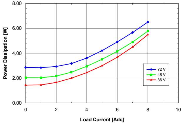
Fig. 6.0V.7: Power dissipation vs. load current and input voltage for SQ48T/S08060 converter mounted vertically with air flowing from pin 3 to pin 1 at a rate of 300 LFM (1.5 m/s) and T_a = 25\text{ }^\circ\text{C} .
