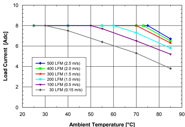
Fig. 6.0V.2: Available load current vs. ambient air temperature and airflow rates for SQ48T08060 converter with D height pins mounted horizontally with V_{in} = 48\text{ V} , air flowing from pin 3 to pin 1, and maximum FET temperature \leq 120\text{ }^\circ\text{C} .
