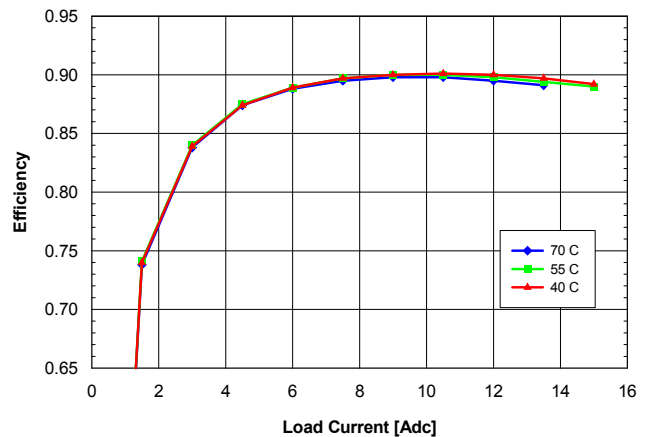
Fig. 3.3V.6: Efficiency vs. load current and ambient temperature for SQ48T/S15033 converter mounted vertically with V_{in} = 48\text{ V} and air flowing from pin 3 to pin 1 at a rate of 200 LFM (1.0 m/s).
