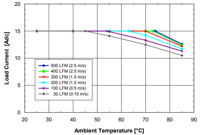
Fig. 3.3V.4: Available load current vs. ambient air temperature and airflow rates for SQ48S15033 converter mounted horizontally with V_{in} = 48\text{ V} , air flowing from pin 3 to pin 1, and maximum FET temperature \leq 120\text{ }^\circ\text{C} .
