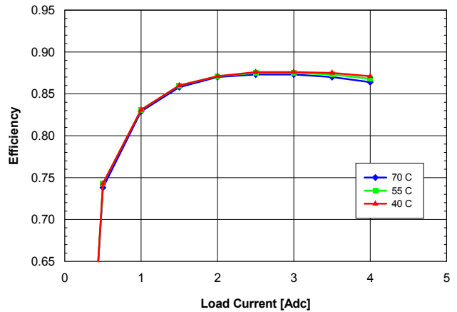
Fig. 12V.6: Efficiency vs. load current and ambient temperature for SQ48T/S04120 converter mounted vertically with V_{in} = 48\text{ V} and air flowing from pin 3 to pin 1 at a rate of 200 LFM (1.0 m/s).
