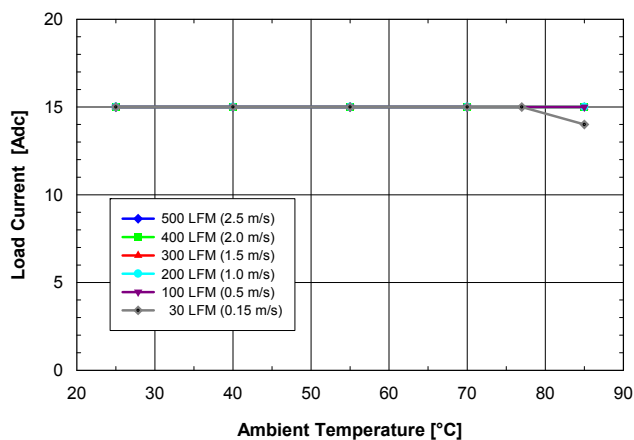
Fig. 1.2V.2: Available load current vs. ambient air temperature and airflow rates for SQ48T15012 converter with D height pins mounted horizontally with V_{in} = 48\text{ V} , air flowing from pin 3 to pin 1, and maximum FET temperature \leq 120\text{ }^\circ\text{C} .
