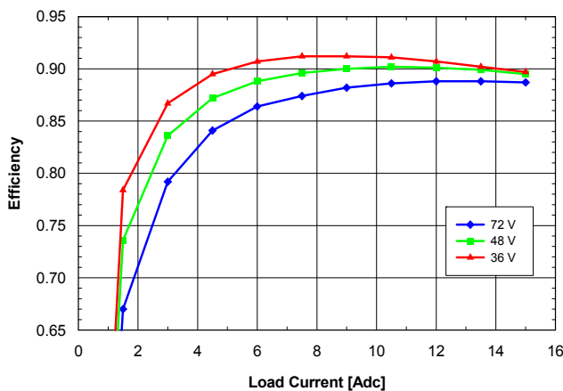
Fig. 3.3V.5: Efficiency vs. load current and input voltage for SQ48T/S15033 converter mounted vertically with air flowing from pin 3 to pin 1 at a rate of 300 LFM (1.5 m/s) and T_a = 25\text{ }^\circ\text{C} .
