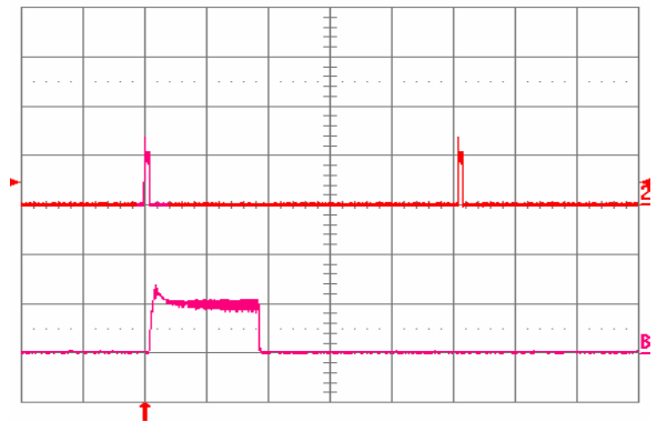
Fig. 12V.18: Load current (top trace, 5 A/div., 20 ms/div.) into a 10 m\Omega short circuit during restart, at V_{in} = 48 V. Bottom trace (5 A/div., 1 ms/div.) is an expansion of the on-time portion of the top trace.
