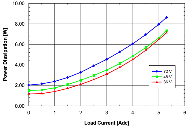
Fig. 8.0V.7: Power dissipation vs. load current and input voltage for SQ48T/S05080 converter mounted vertically with air flowing from pin 3 to pin 1 at a rate of 300 LFM (1.5 m/s) and T_a = 25\text{ }^\circ\text{C} .
